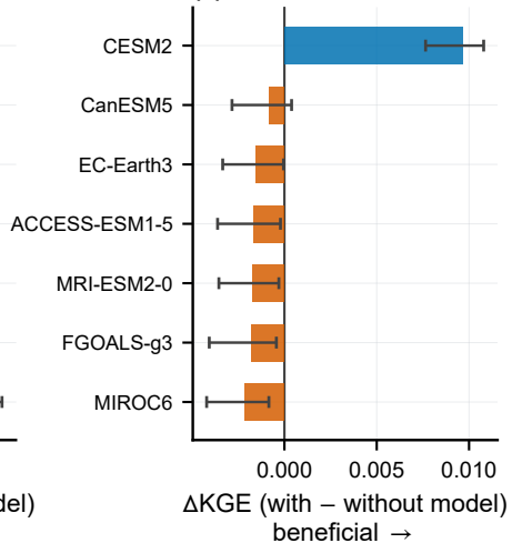
(c) Model influence — KGE
