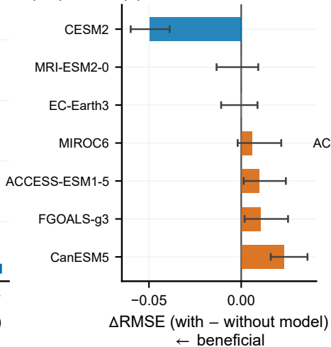
(b) Model influence — RMSE
