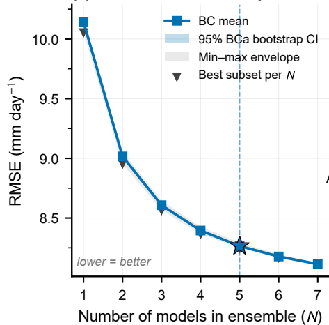
(a) Sub-ensemble envelope — RMSE (BC)
